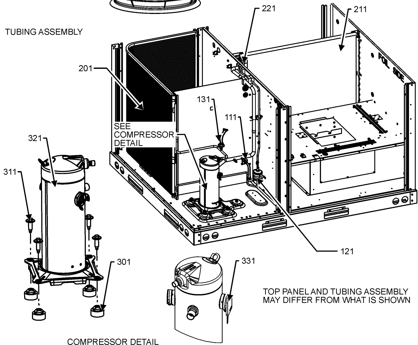
COMPRESSOR DETAIL
