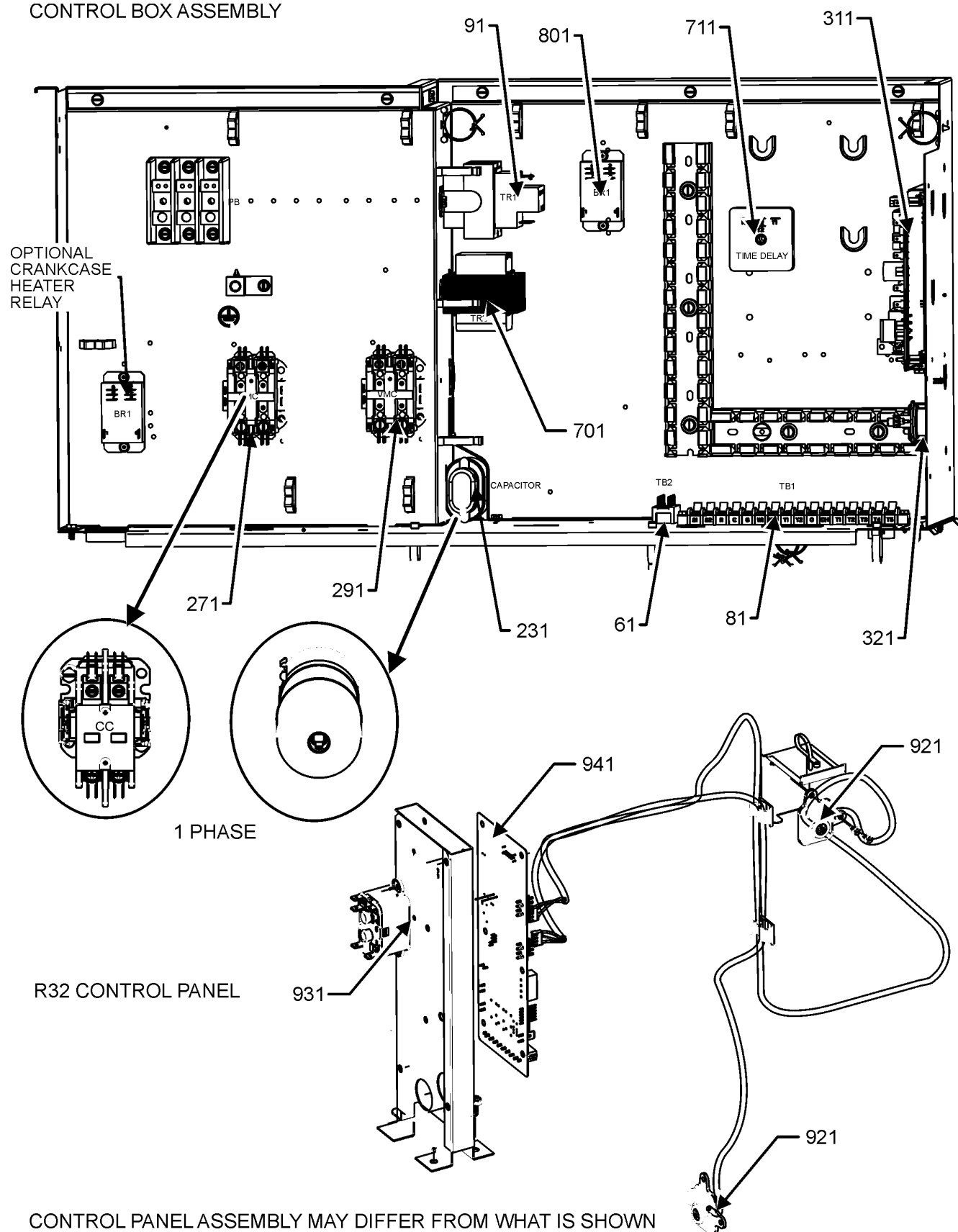
CONTROL BOX ASSEMBLY
