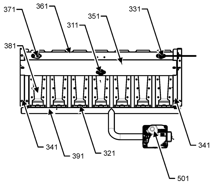
MANIFOLD ASSEMBLY
