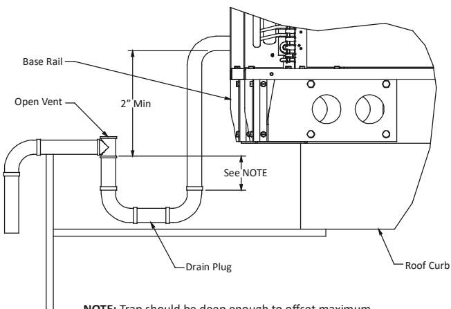
Drain Pan (Side View)
