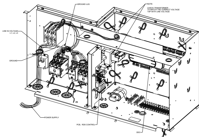
HP/AC DDC CONTROL BOX
