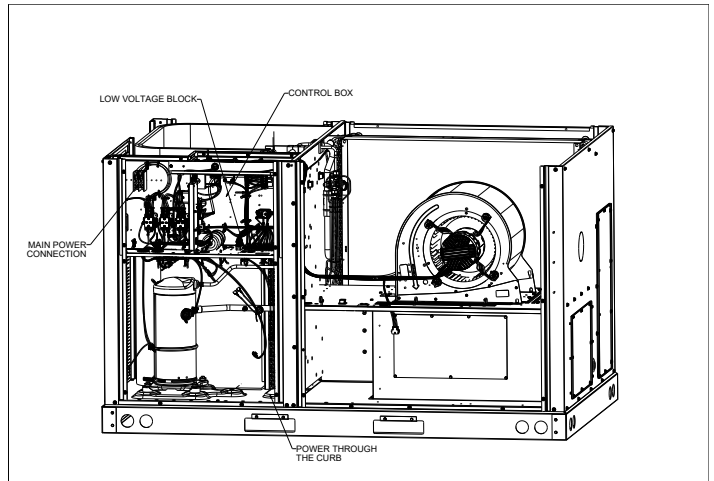
HP/AC UNIT
