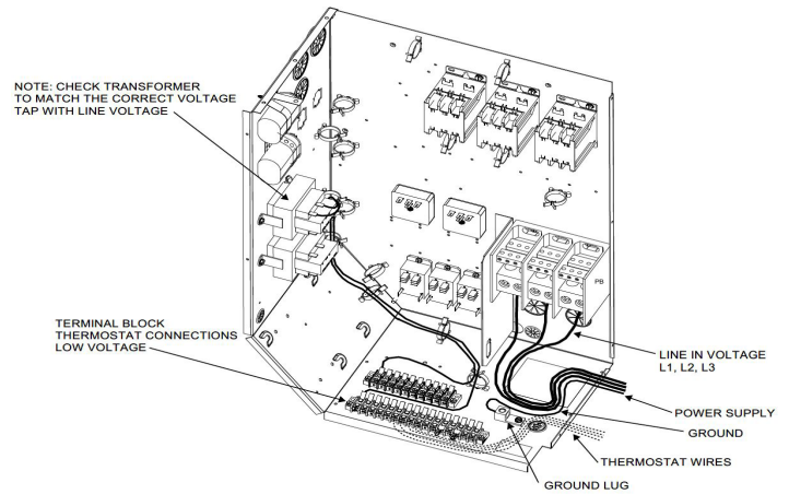
Thermostat Control Box
