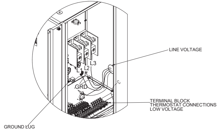
Thermostat Control Box
