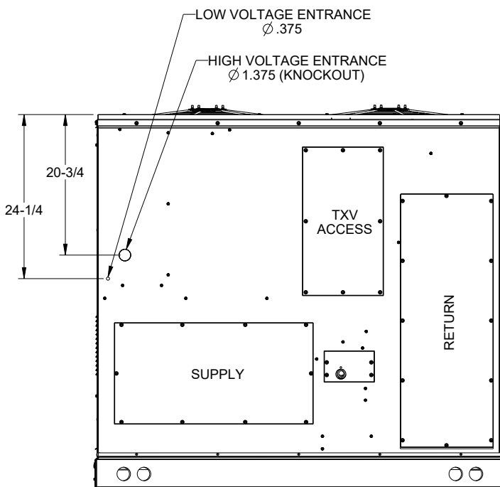
Thermostat Duct Panel
