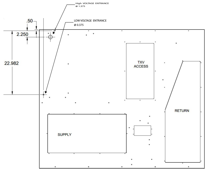
DDC Duct Panel
