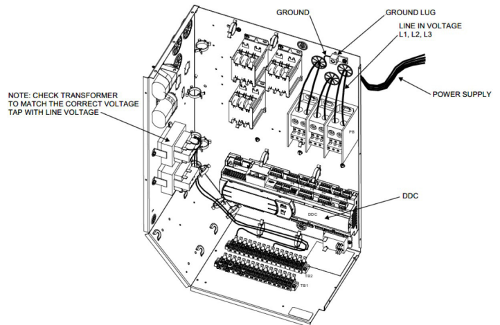
DDC Control Box
