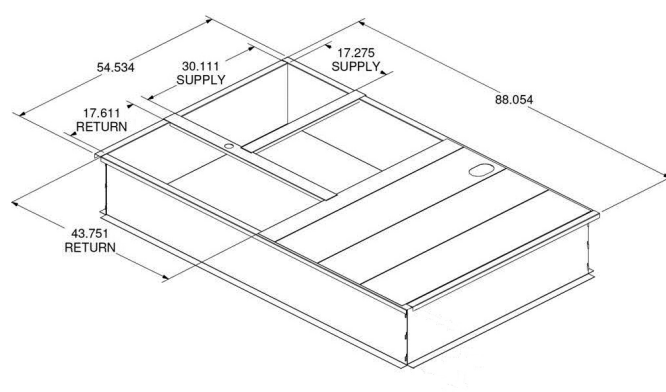
7.5-12.5 Ton Roof Curb Footprint
