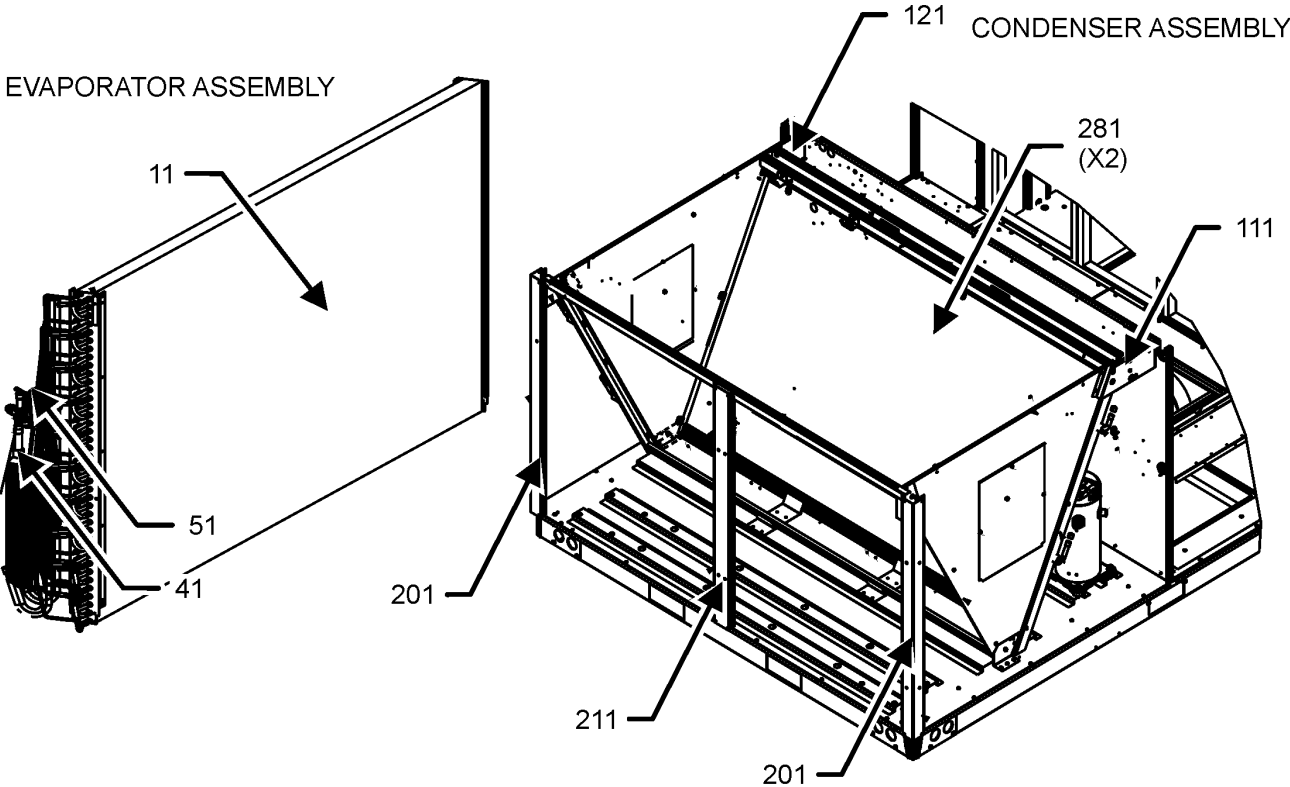
PARTITION, EVAPORATOR, CONDENSER ASSEMBLY
