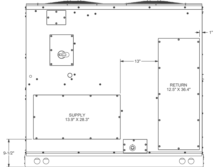
HORIZONTAL DISCHARGE DUCT CONNECTIONS FIGURE 3
