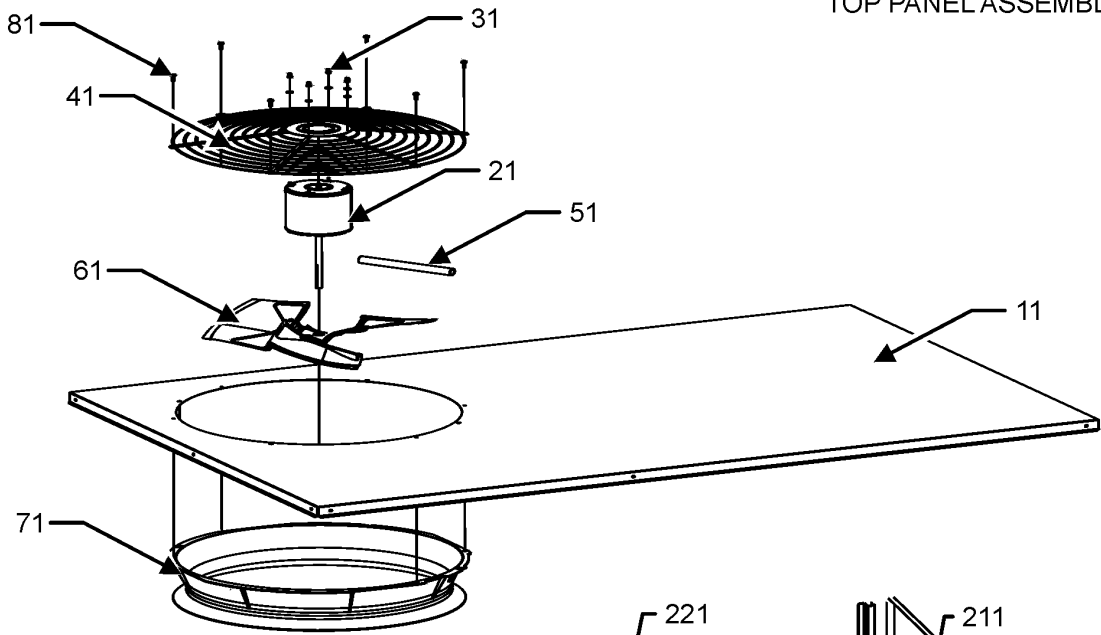
TUBING ASSEMBLY
