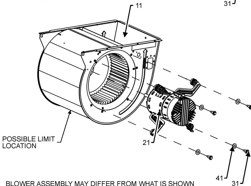
BLOWER ASSEMBLY 2
