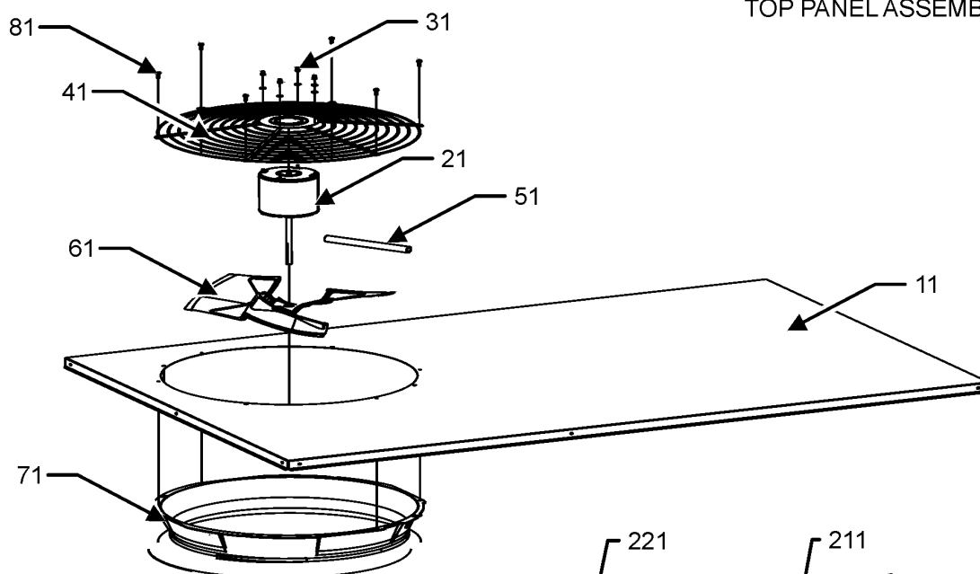
TUBING ASSEMBLY
