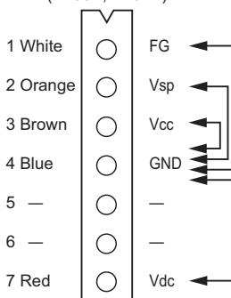
Connector for signal wires (X106A, X107A)
