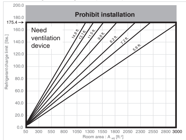
◆ Total refrigerant charge limit (FPS unit)
