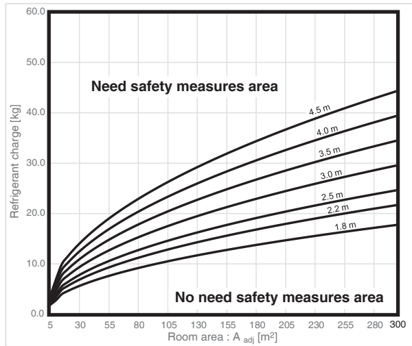
◆ Safety measures required or not (SI unit)
