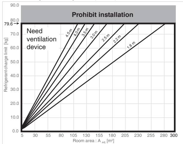
◆ Total refrigerant charge limit (SI unit)
