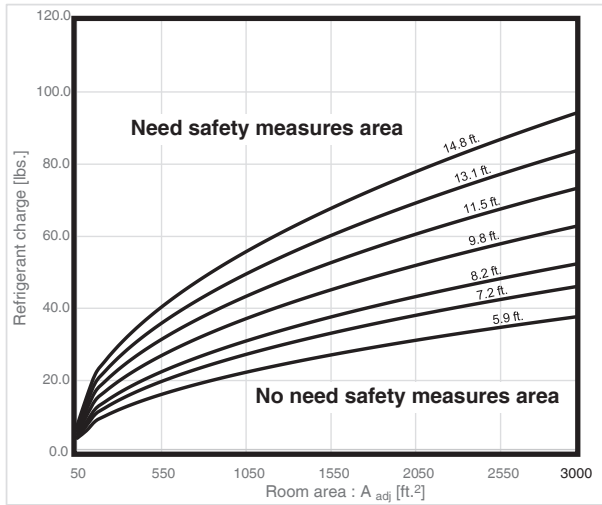
◆ Safety measures required or not (FPS unit)
